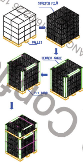
TWO PALLET SHIPMENT EXAMPLE SHIPPING BY SEA USFD
