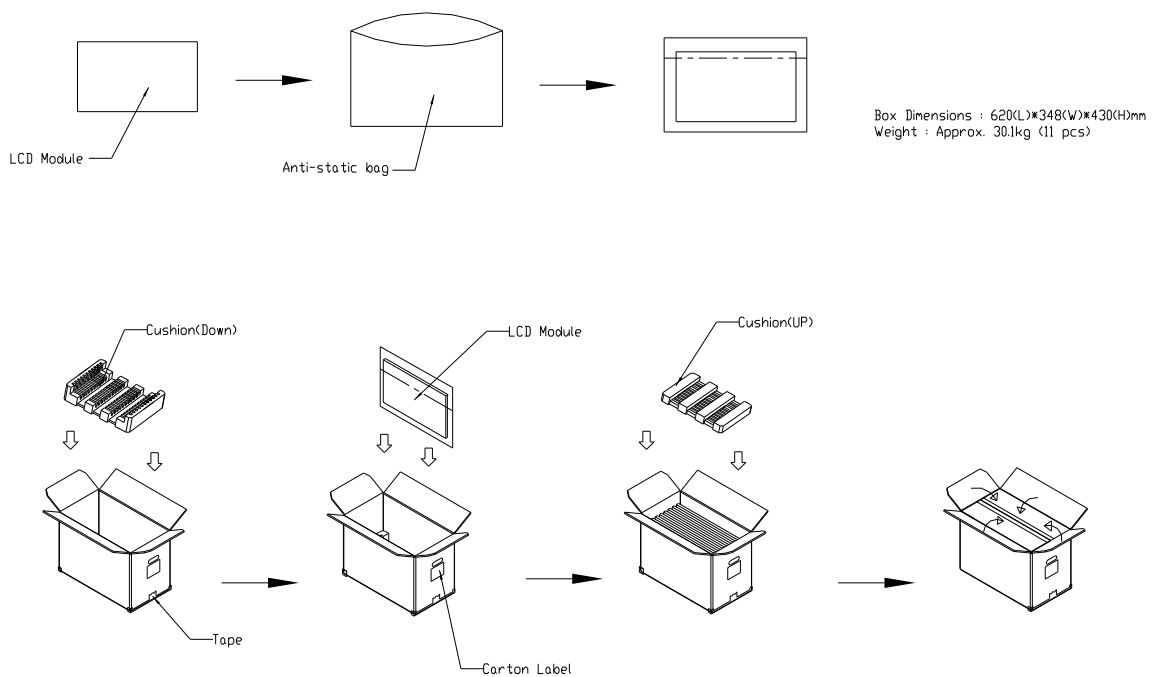
Figure. 8-1 Packing method
