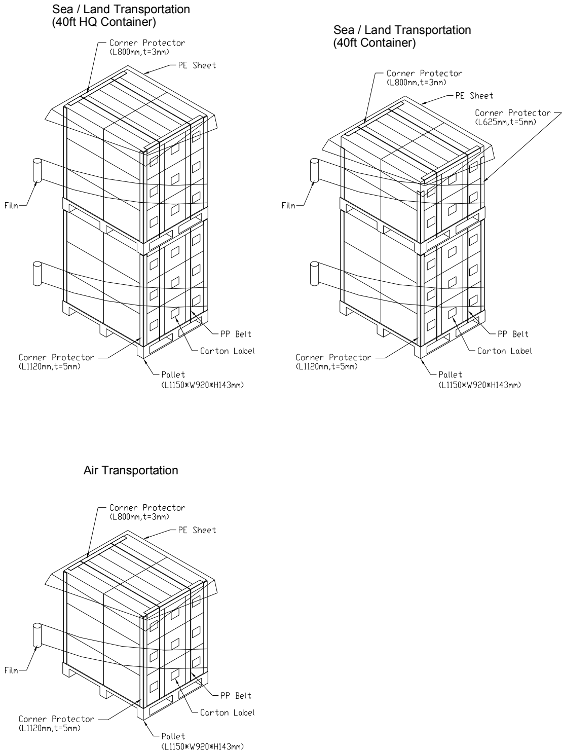
Figure. 8-2 Packing method
