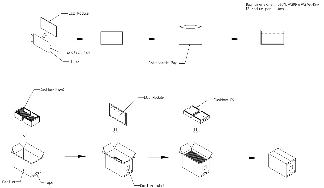
Figure. 8-1 Packing method
