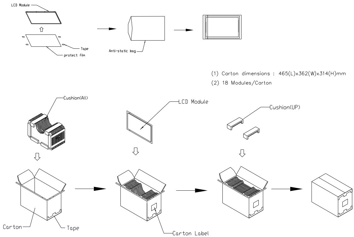
Figure. 9-1 Packing method
