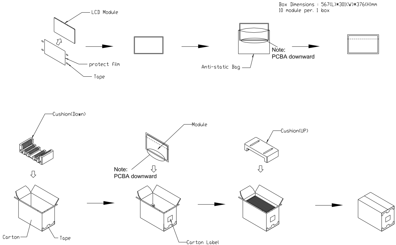
Figure. 8-1 Packing method
