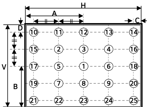
<Measuring point for luminance variation>
