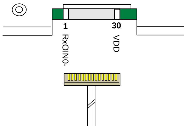
LVDS Connector (CN1)
