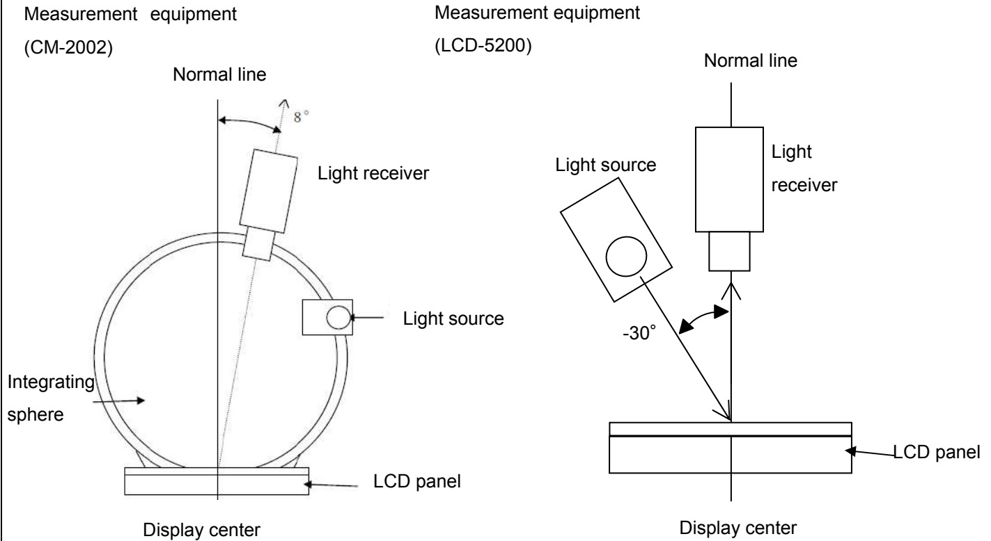
Fig7-2 Contrast ratio, Reflection ratio, Panel chromaticity of white
