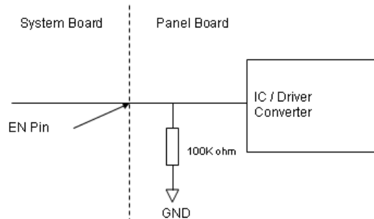
BLON Pin
