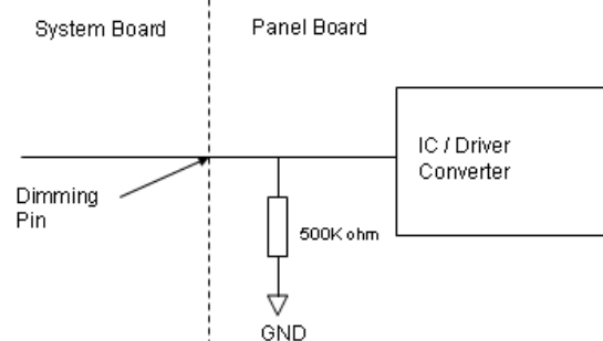
E_PWM Pin
